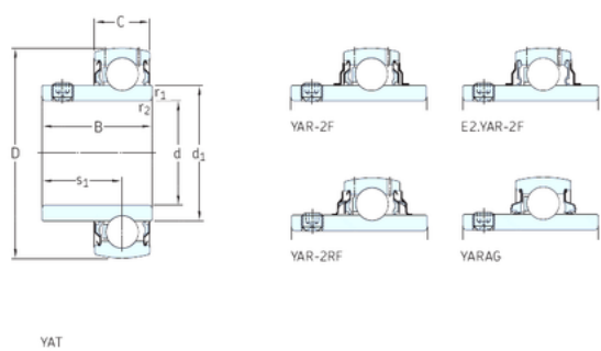
Bearing No. YAR206-102-2F
