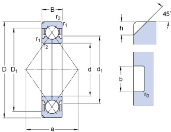
Bearing No. QJ 306 N2PHAS
