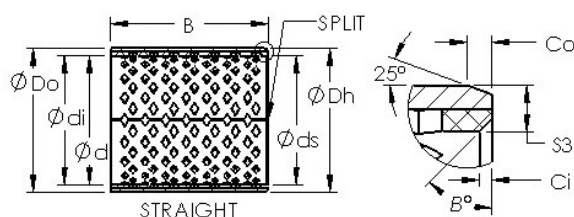
Bearing No. AST090 17080
