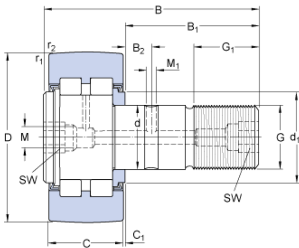
Bearing No. PWKR 40.2RS
