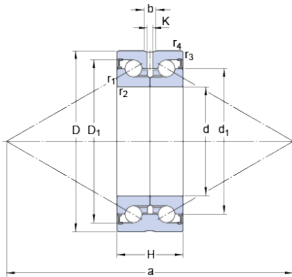
Bearing No. BEAS 020052-2RZ/PE
