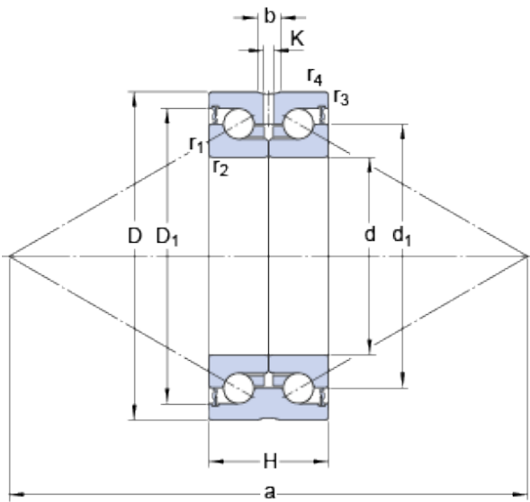
Bearing No. BEAS 017047-2RS
