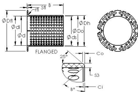
Bearing No. ASTT90 F5550
