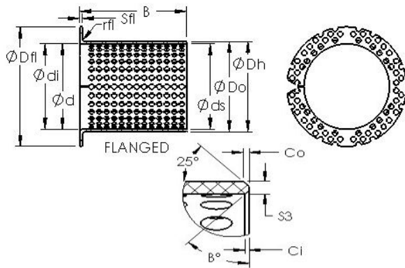
Bearing No. ASTT90 F4550
