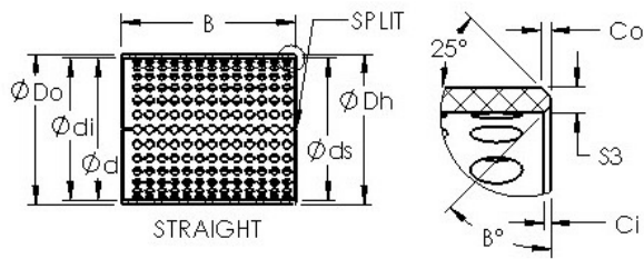
Bearing No. ASTT90 7540
