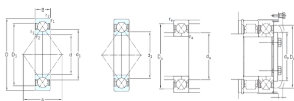
Bearing No. QJ306MA
