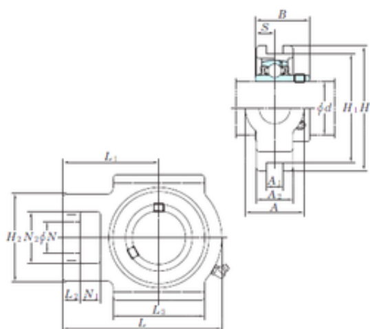
Bearing No. UCT210
