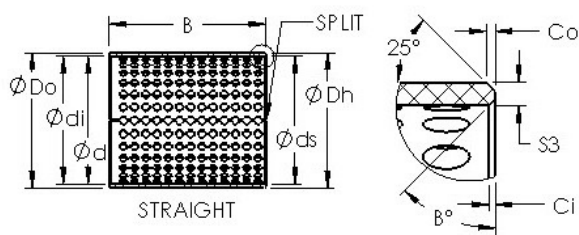
Bearing No. ASTT90 13560
