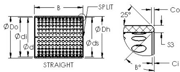
Bearing No. ASTT90 11050
