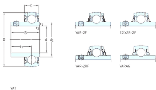
Bearing No. YAR217-2F
