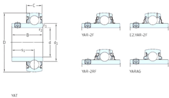
Bearing No. YAR209-2F
