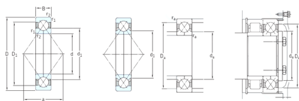
Bearing No. QJ330N2MA
