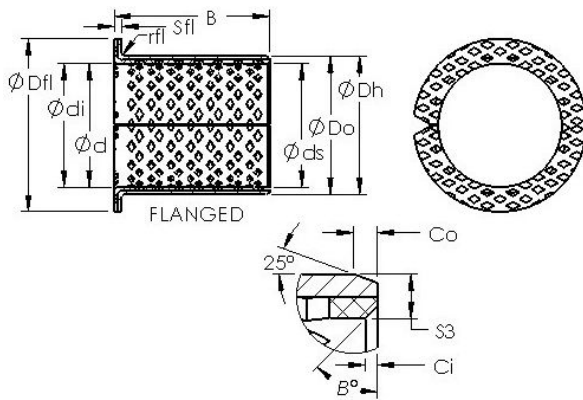
Bearing No. ASTB90 F6050
