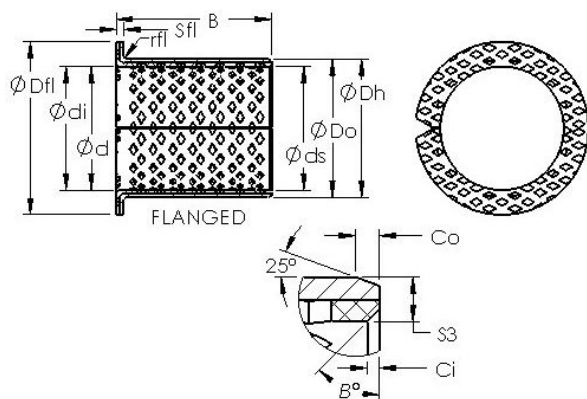
Bearing No. ASTB90 F5540
