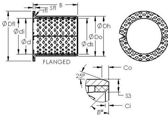
Bearing No. ASTB90 F4540
