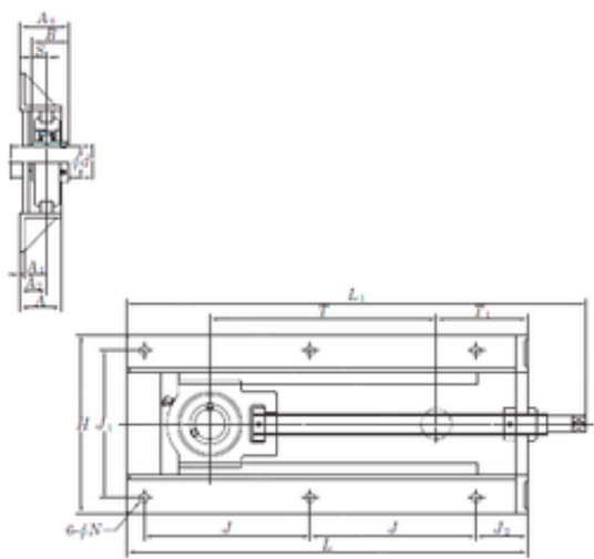
Bearing No. UCTH207-20-230
