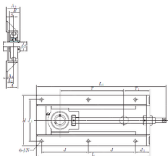
Bearing No. UCTH202-150
