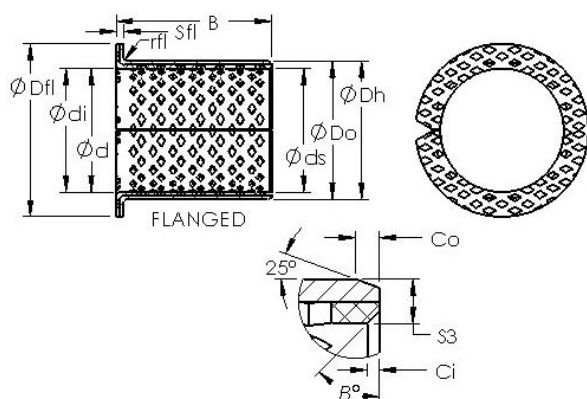
Bearing No. ASTB90 F12060
