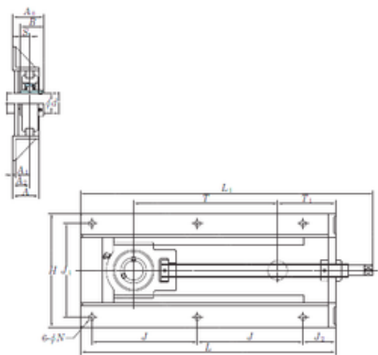
Bearing No. UCTH209-26-300
