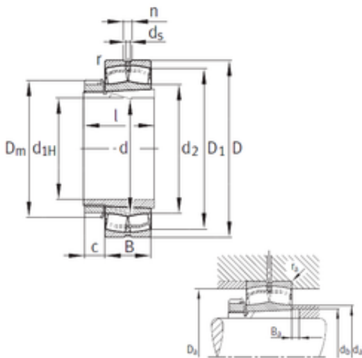
Bearing No. 22238-K-MB+H3138
