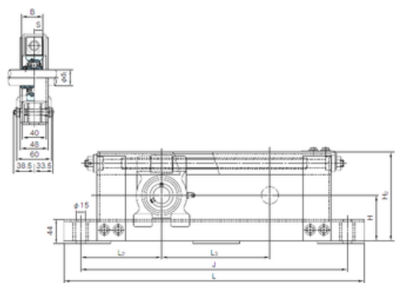
Bearing No. UCTL207+WL400
