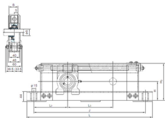
Bearing No. UCTL205+WL400
