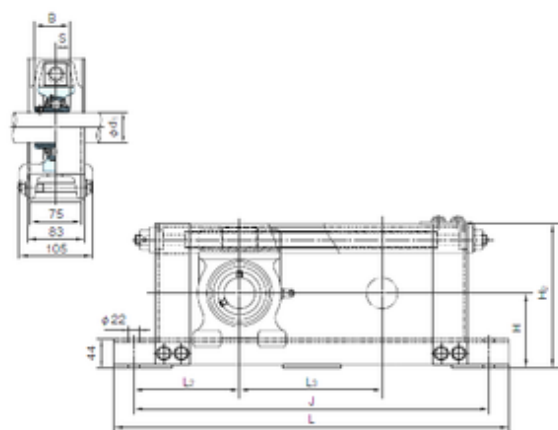
Bearing No. UCTU208+WU900
