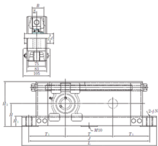
Bearing No. UCTU212-900
