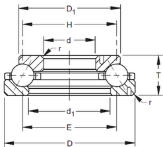
Bearing No. 170TVL500
