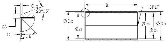
Bearing No. AST850BM 3220
