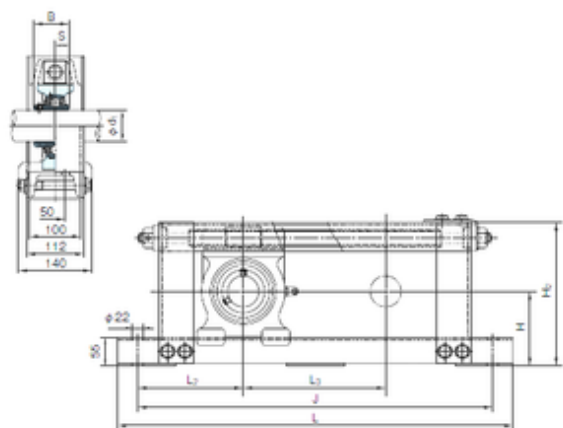
Bearing No. UCTU318+WU700
