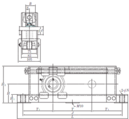
Bearing No. UCTU317-800
