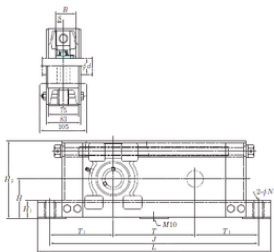
Bearing No. UCTU318-700
