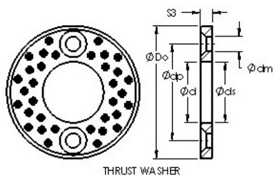
Bearing No. AST650 WC60
