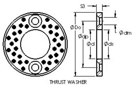
Bearing No. AST650 WC55
