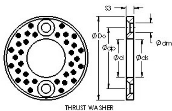
Bearing No. AST650 WC16N
