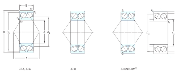
Bearing No. 3308ATN9
