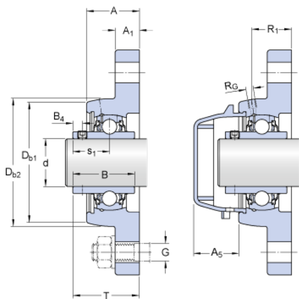
Bearing No. FYTWR 25 YTHR
