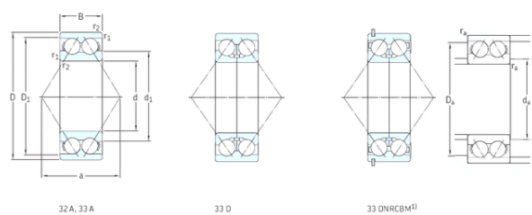
Bearing No. 3306ATN9
