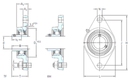
Bearing No. FYTJ 1.1/2 TF
