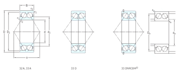
Bearing No. 3305ATN9
