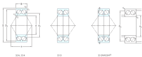
Bearing No. 3304ATN9
