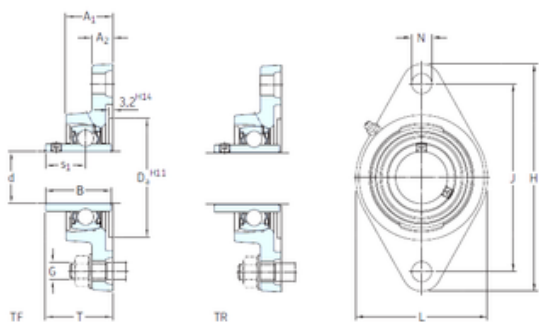
Bearing No. FYTB 20 TF
