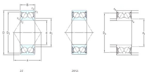
Bearing No. 3303A-2Z
