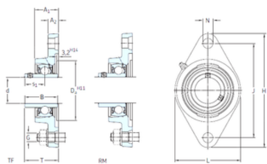
Bearing No. FYT 1.7/16 TF
