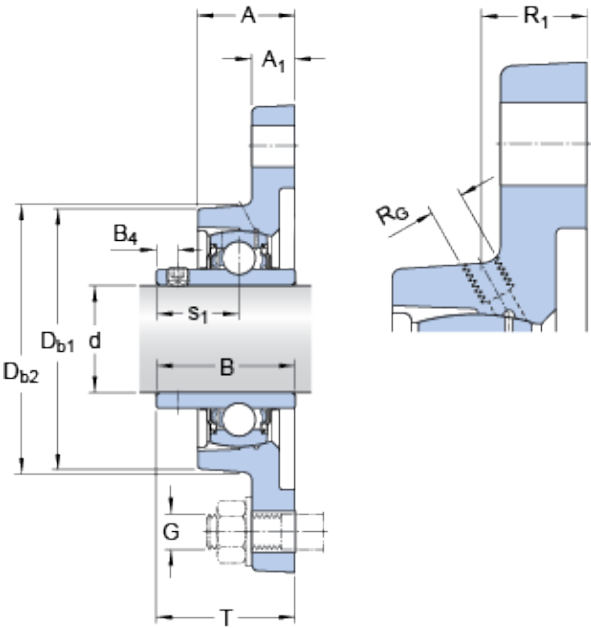
Bearing No. FYT 1.3/4 TF
