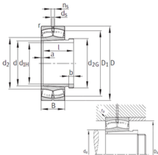
Bearing No. 24128-E1-K30+AH+AH24128
