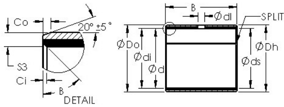
Bearing No. AST50 58IB64
