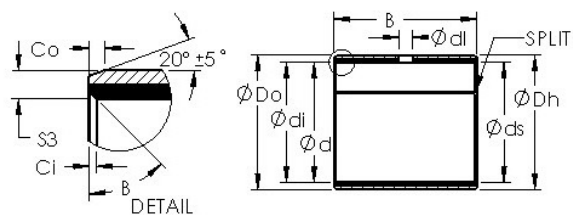
Bearing No. AST50 58IB32
