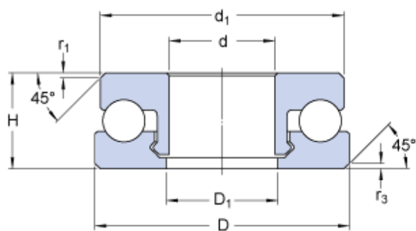
Bearing No. 51109 V/HR22Q2
